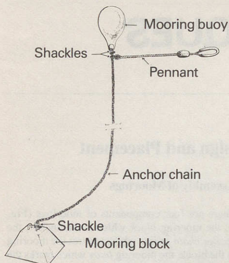
Fig. 1. Diagram of a standard mooring
