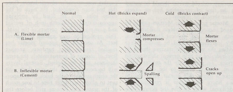
Figure 2. Diagrammatic sketches showing effects of temperature change upon masonry. Flexible mortar (A) expands and contracts with temperature changes. Bricks bonded by inflexible mortar (B) tend to spall at the edges (the area of greatest stress) in hot weather and separate from the mortar when it is cold. This latter condition opens cracks, permitting the entry of water and causing additional deterioration. Adapted from Maintenance of Old Buildings, Document D 10; National Swedish Institute for Building Research, Stockholm, 1975.
