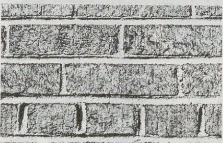
F Concave joint, common bond early 20th century.
