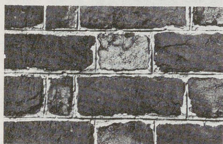
A Colonial grapevine joint, Flemish Bond ca. 1720.
