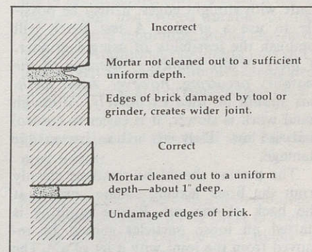
Figure 3. Comparison of incorrect and correct preparation of mortar joints for repointing.
