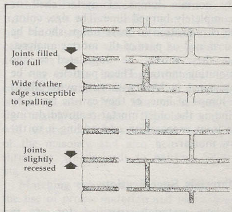
Figure 5. Comparison of visual effect of full mortar joints vs. slightly recessed joints. Filling joints too full hides the actual joint thickness and changes the character of the original brickwork.
